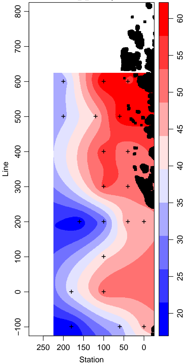
LMG11-01_1_Silicate \mu\text{ mol L}^{-1}
