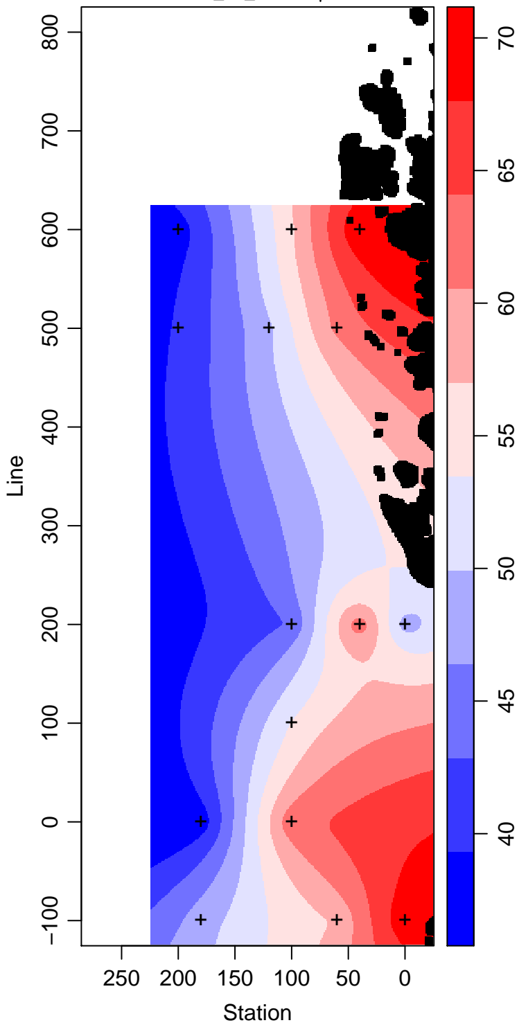
LMG11-01_55_Silicate \mu\text{ mol L}^{-1}
