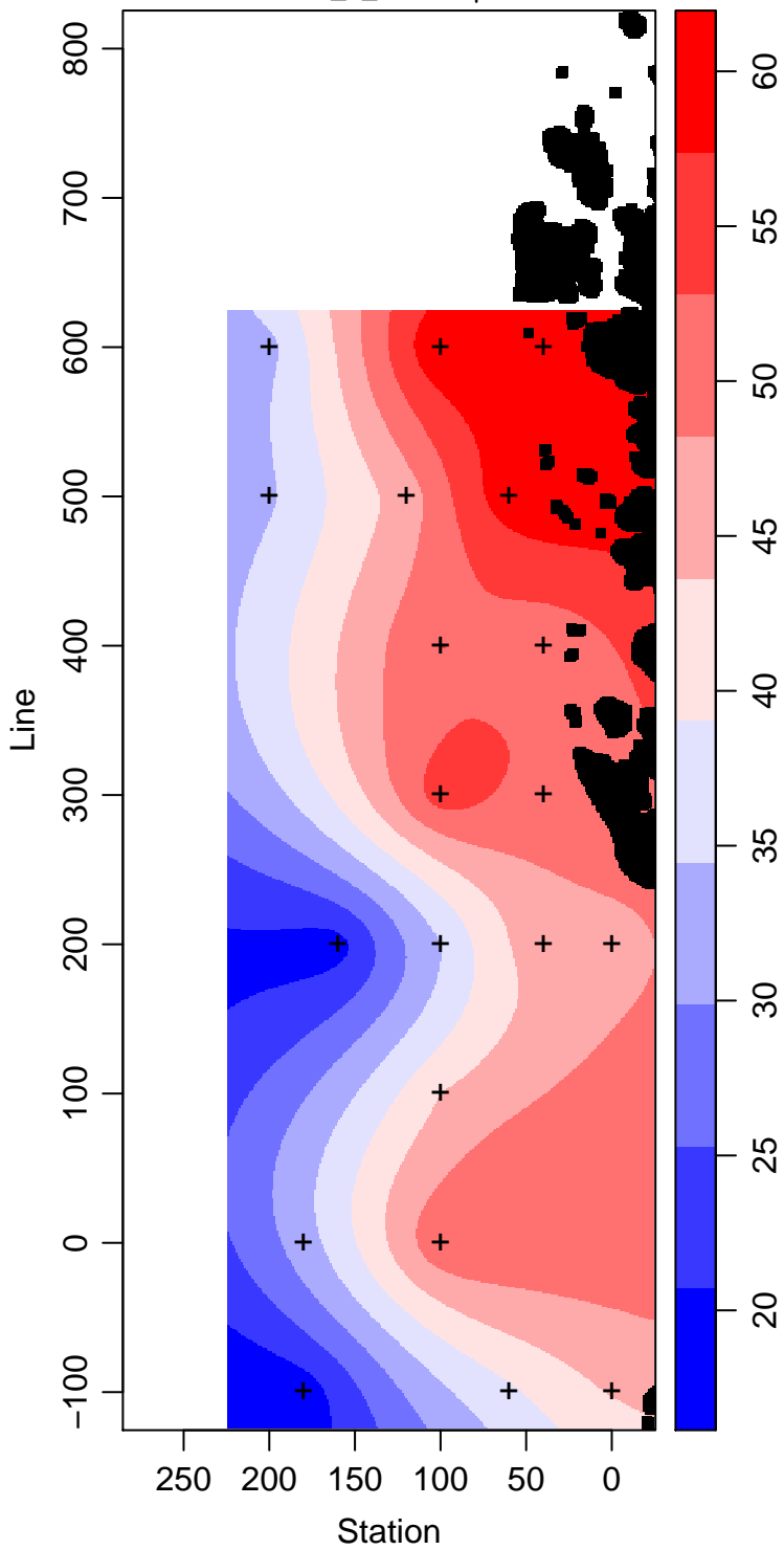
LMG11-01_5_Silicate \mu\text{ mol L}^{-1}
