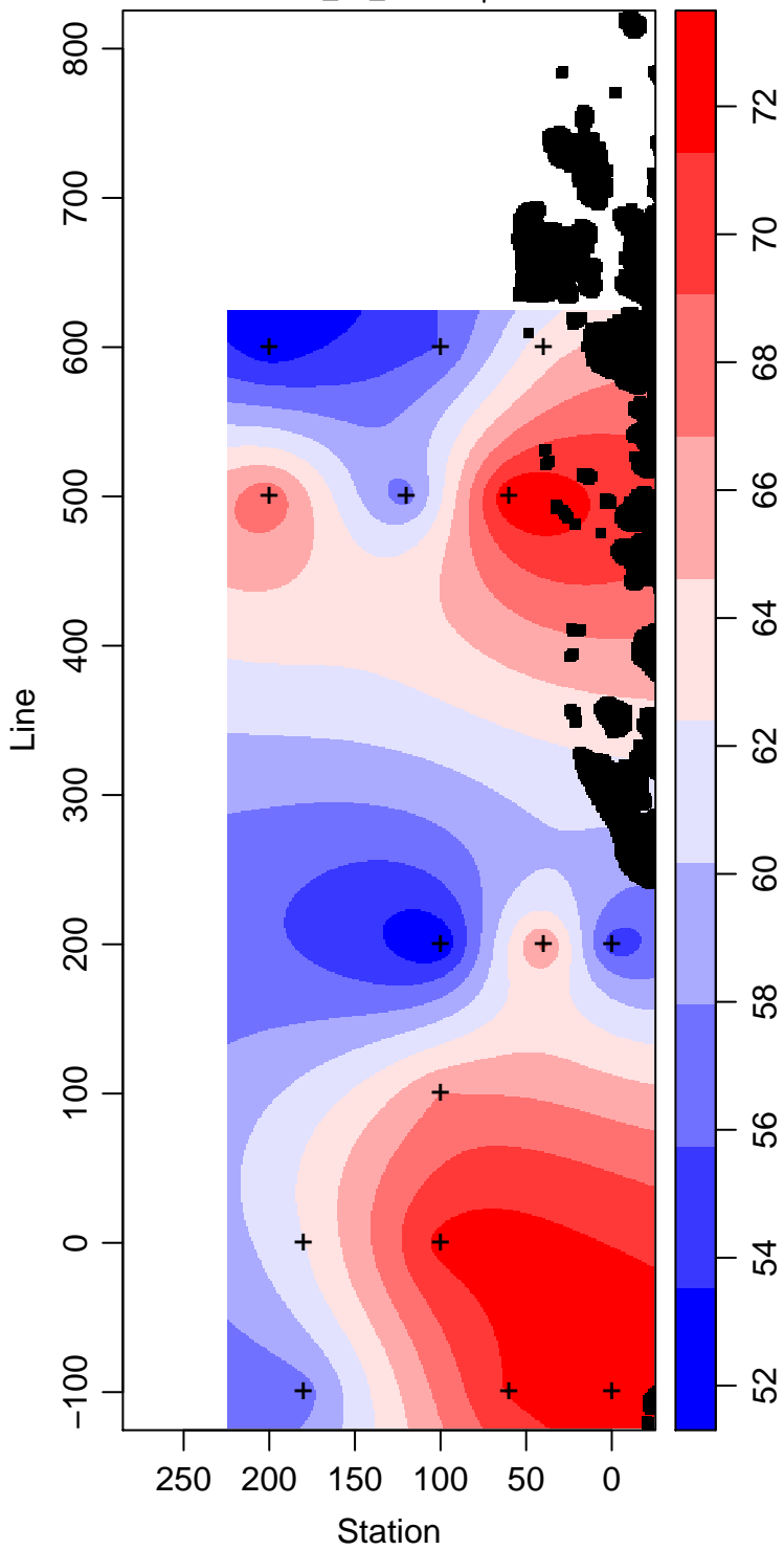
LMG11-01_95_Silicate \mu\text{ mol L}^{-1}
