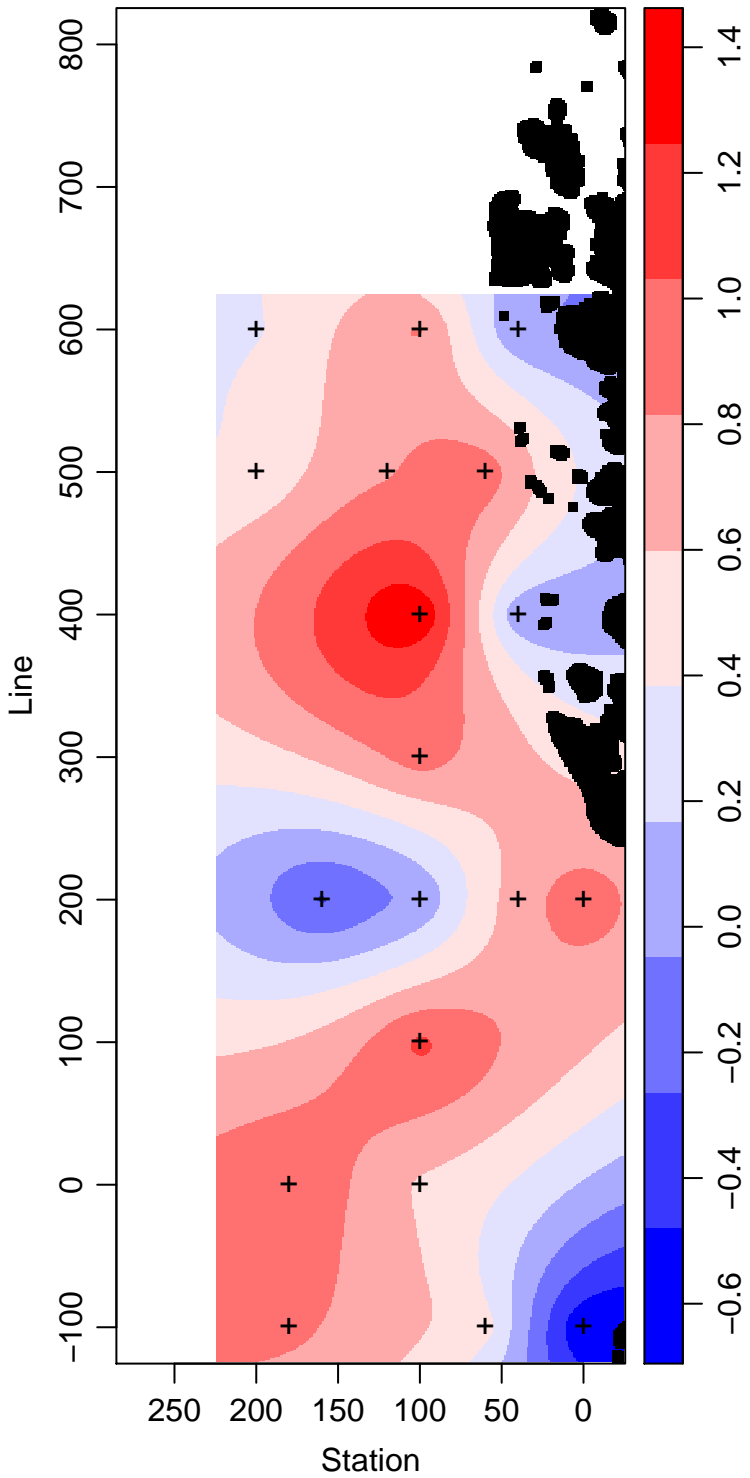
LMG11-01_25_Temperature ° Celsius
