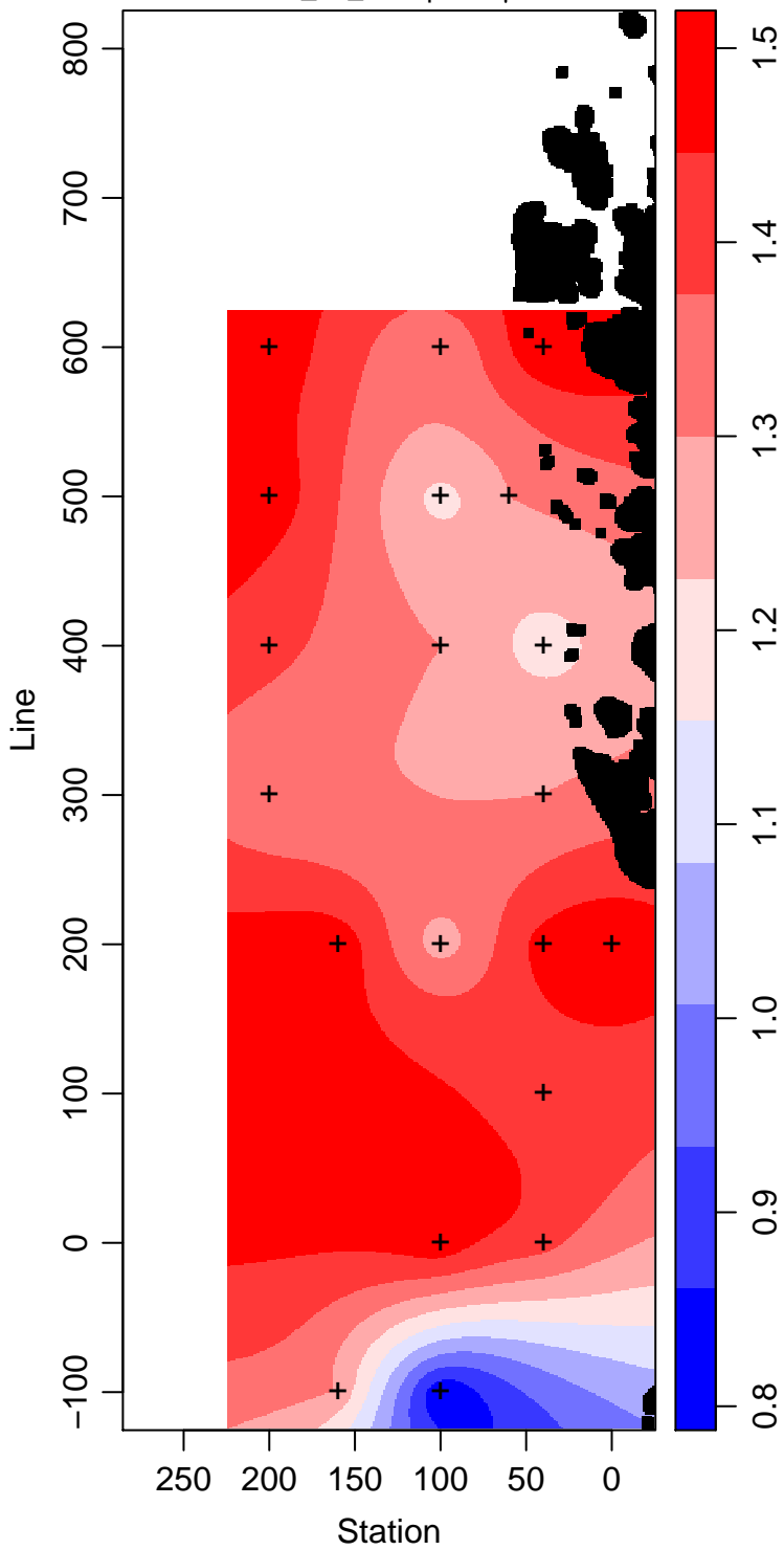
LMG12-01_10_Phosphate \mu\text{ mol L}^{-1}
