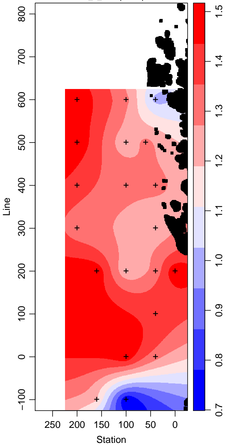
LMG12-01_1_Phosphate \mu\text{ mol L}^{-1}
