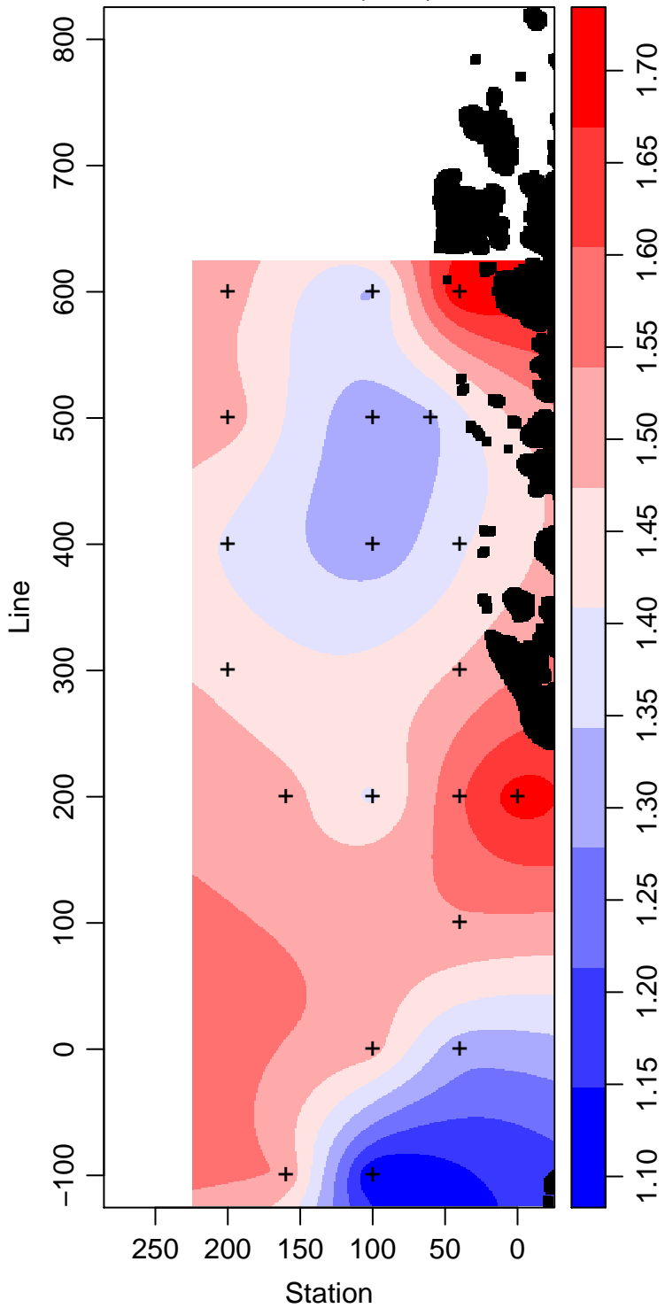
LMG12-01_20_Phosphate \mu\text{ mol L}^{-1}
