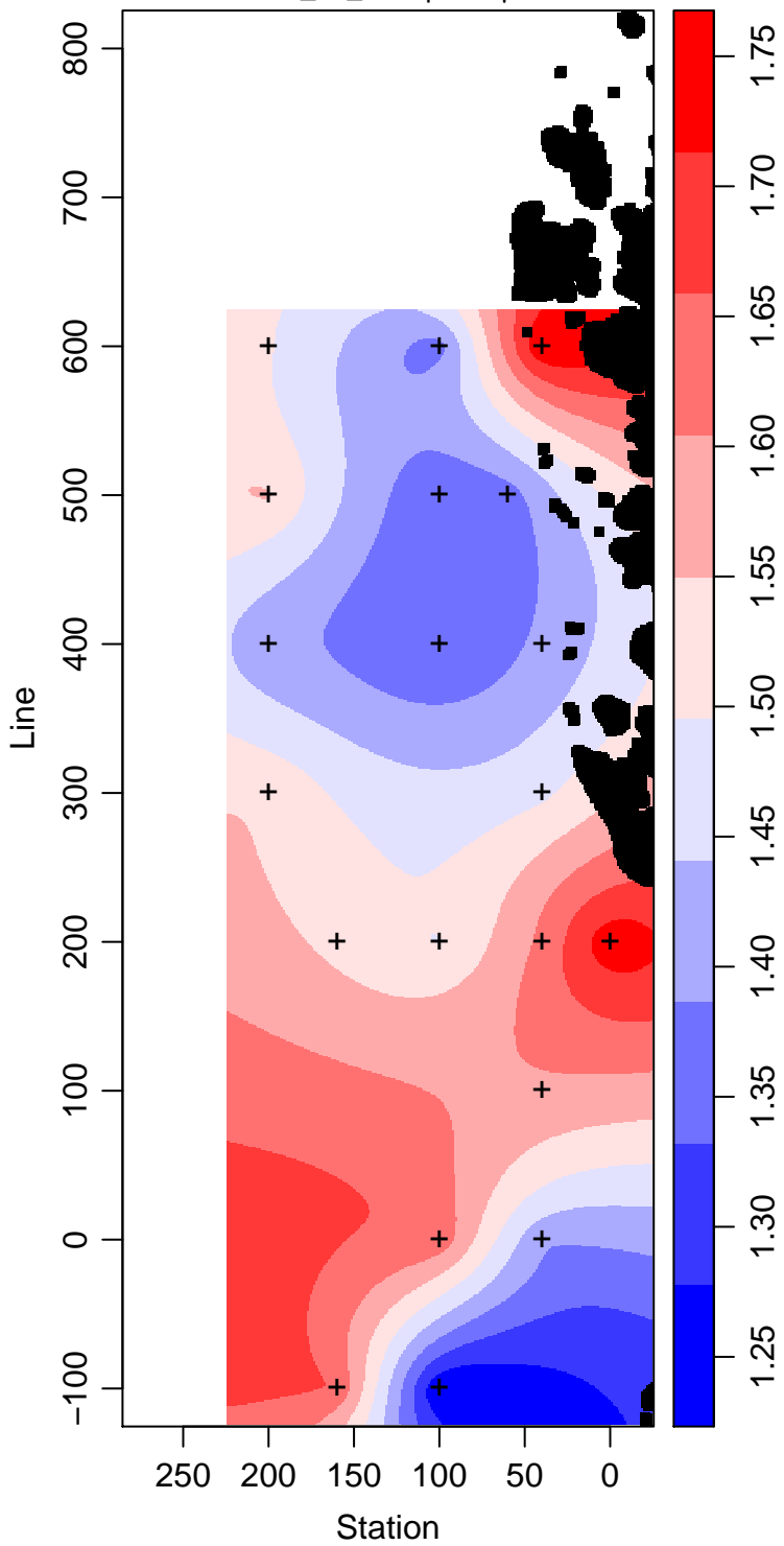
LMG12-01_25_Phosphate \mu\text{ mol L}^{-1}
