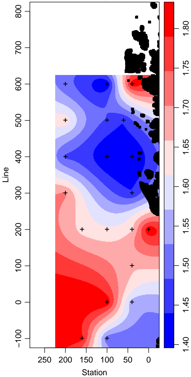
LMG12-01_35_Phosphate \mu\text{ mol L}^{-1}
