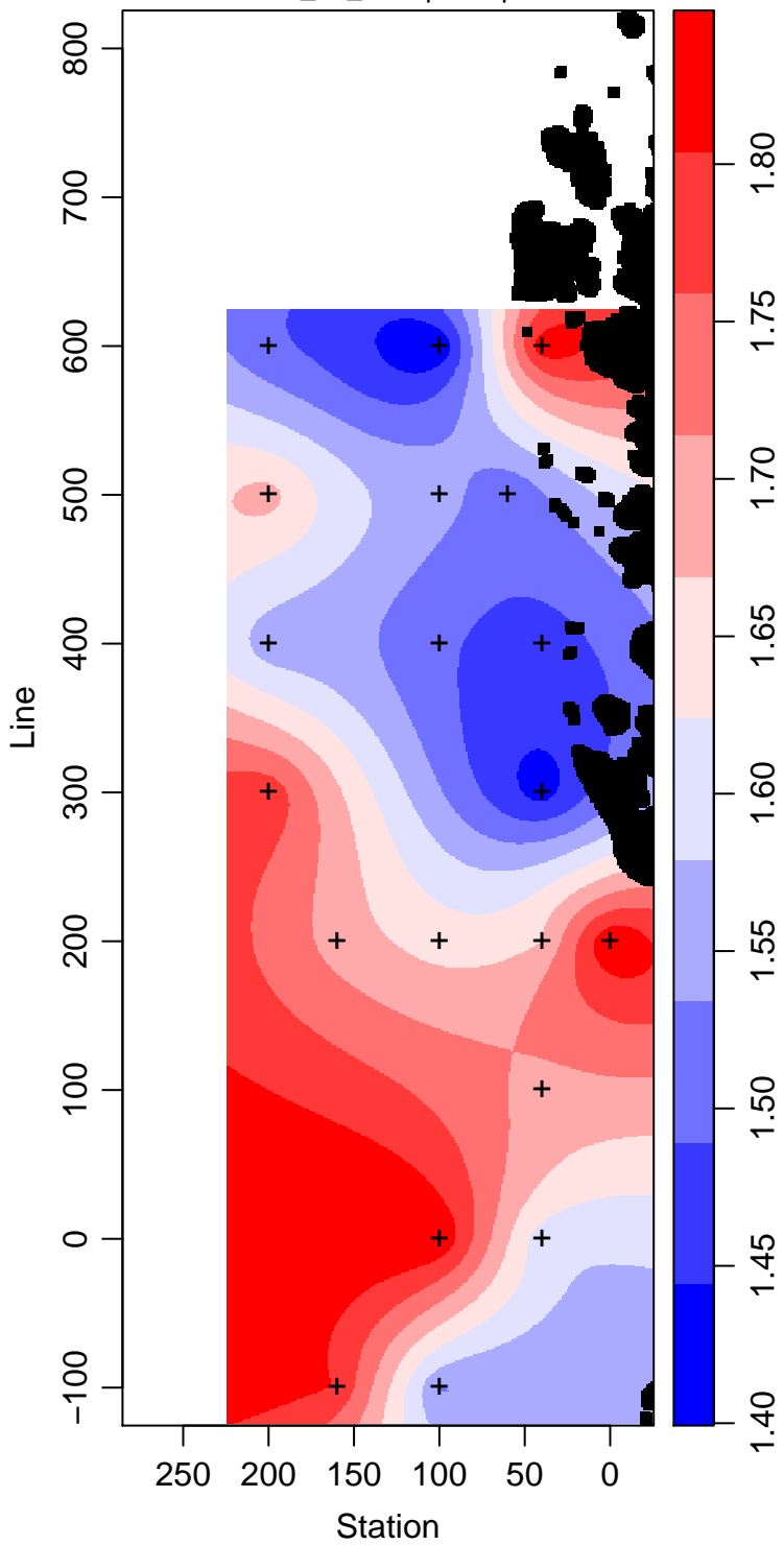
LMG12-01_40_Phosphate \mu\text{ mol L}^{-1}
