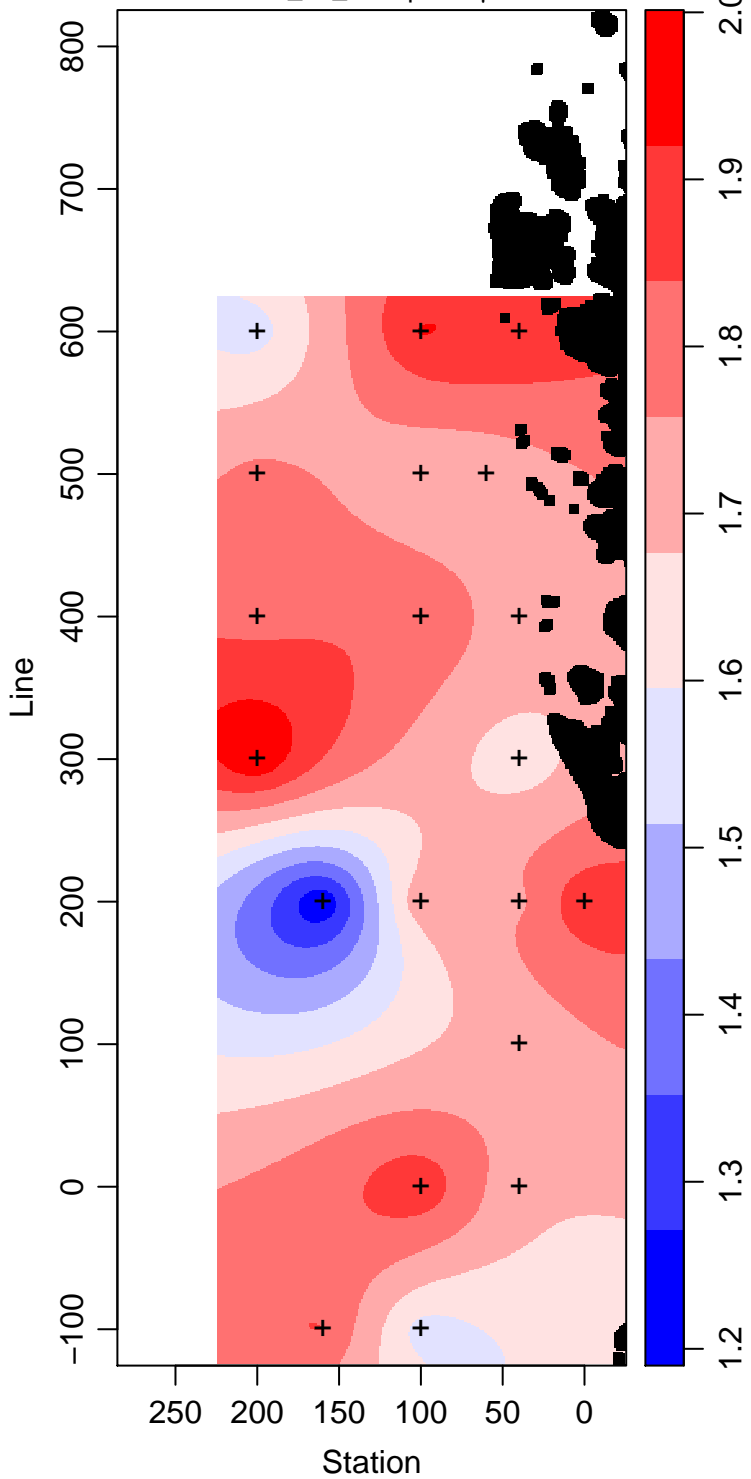
LMG12-01_60_Phosphate \mu\text{ mol L}^{-1}
