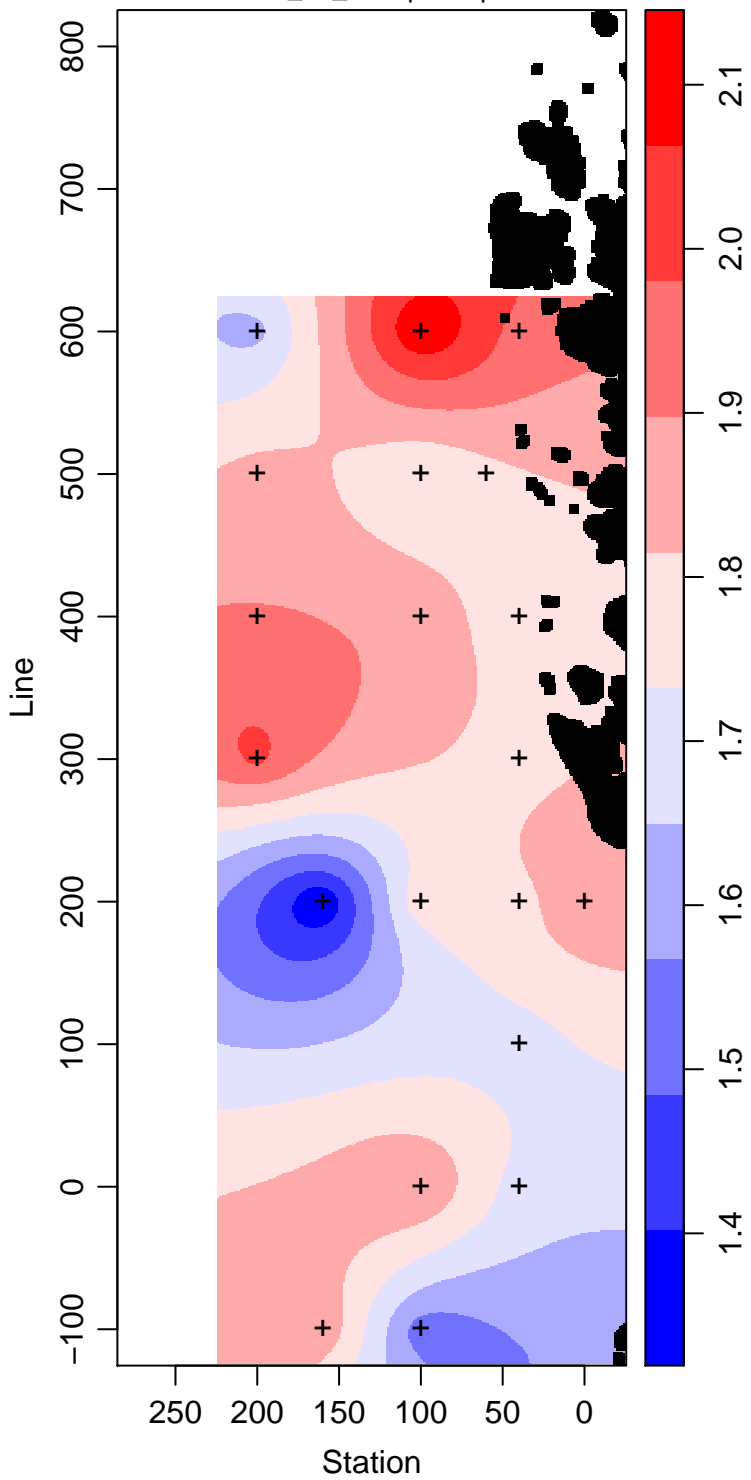
LMG12-01_70_Phosphate \mu\text{ mol L}^{-1}
