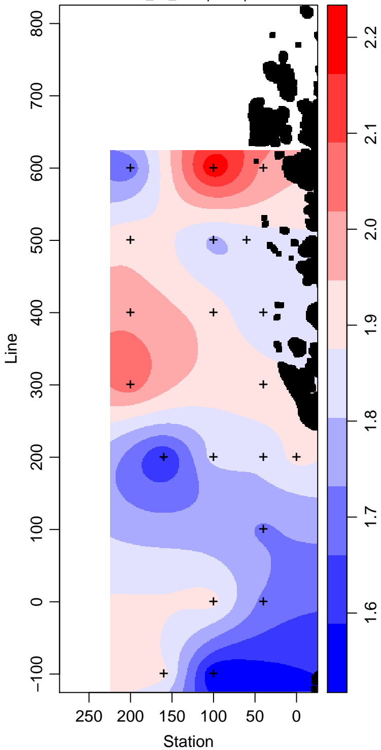
LMG12-01_80_Phosphate \mu\text{ mol L}^{-1}
