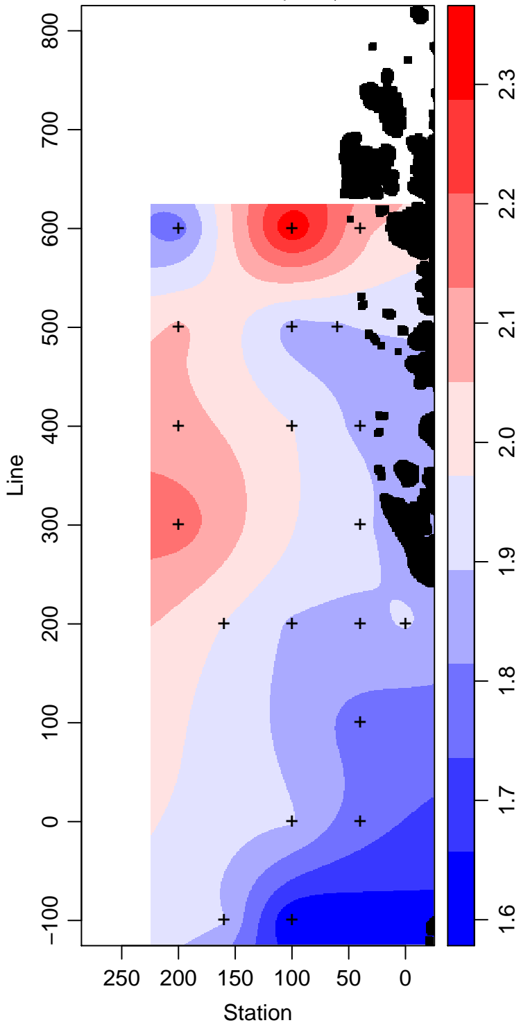
LMG12-01_95_Phosphate \mu\text{ mol L}^{-1}
