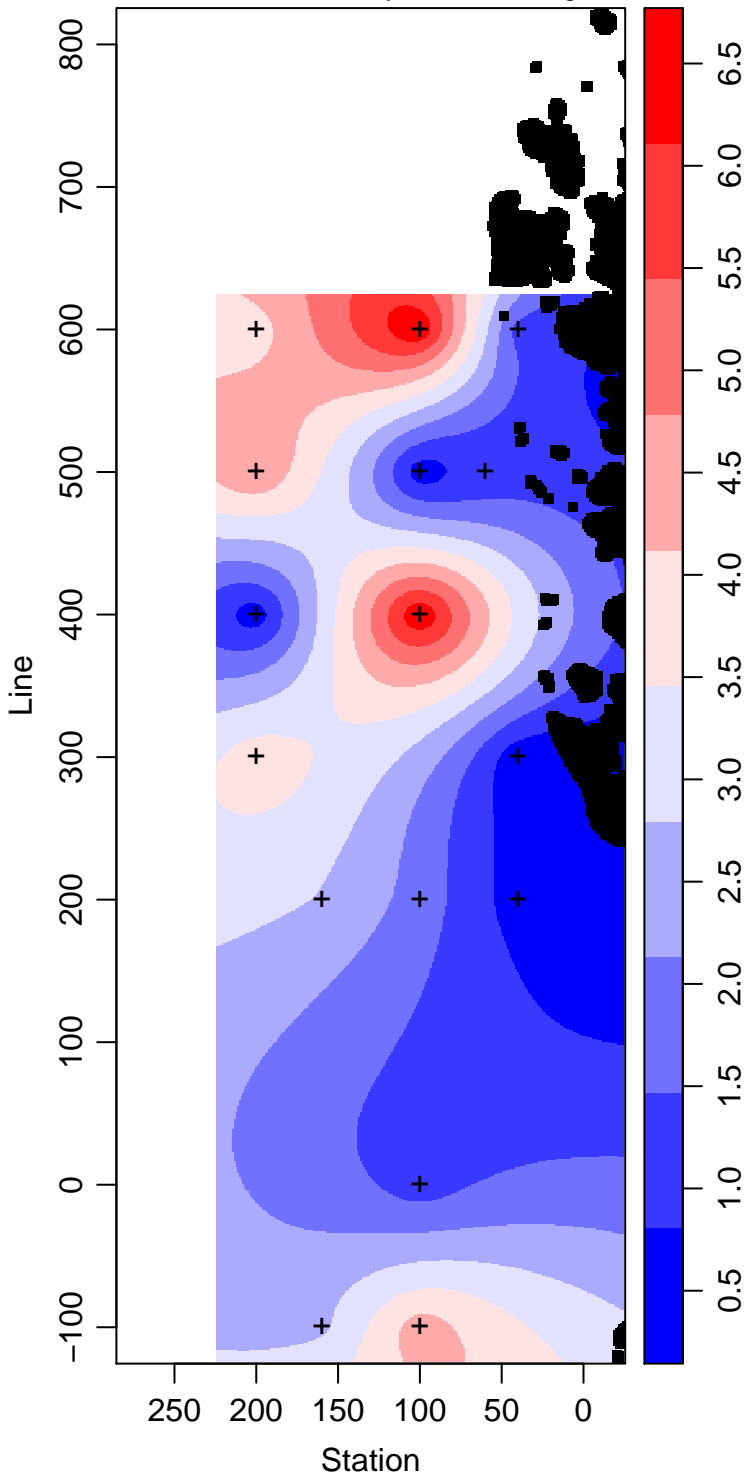
LMG12-01_45_Primary.Production mg m -3
