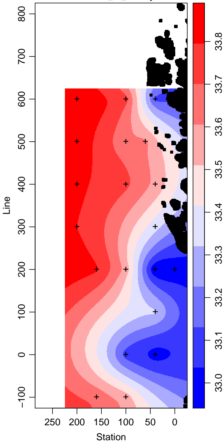
LMG12-01_10_Salinity
