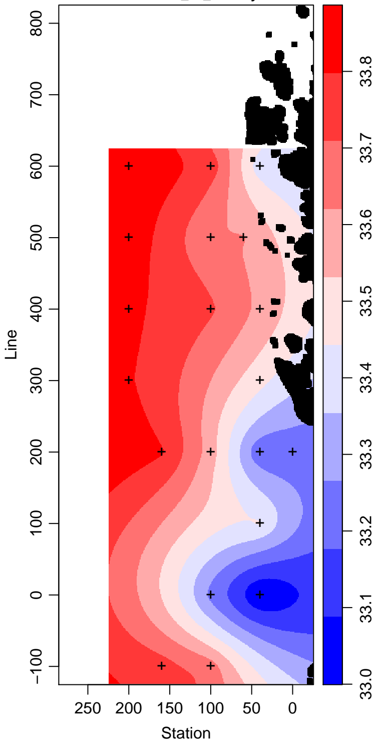
LMG12-01_15_Salinity
