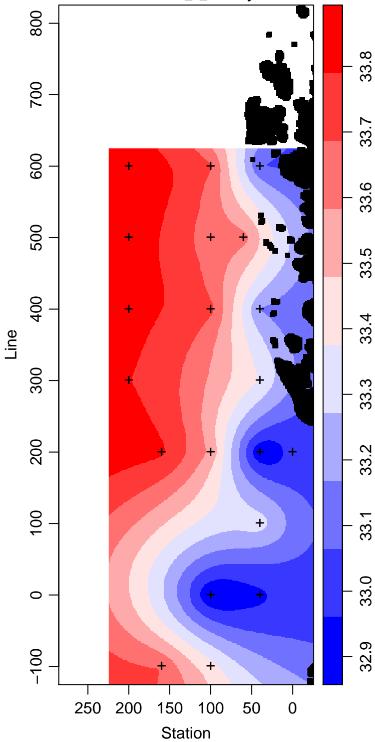
LMG12-01_1_Salinity
