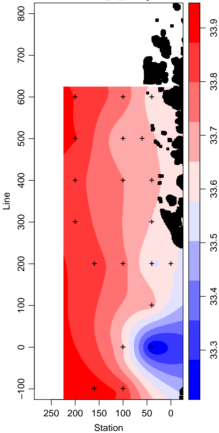
LMG12-01_25_Salinity
