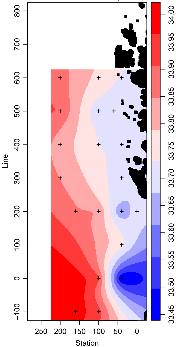
LMG12-01_30_Salinity
