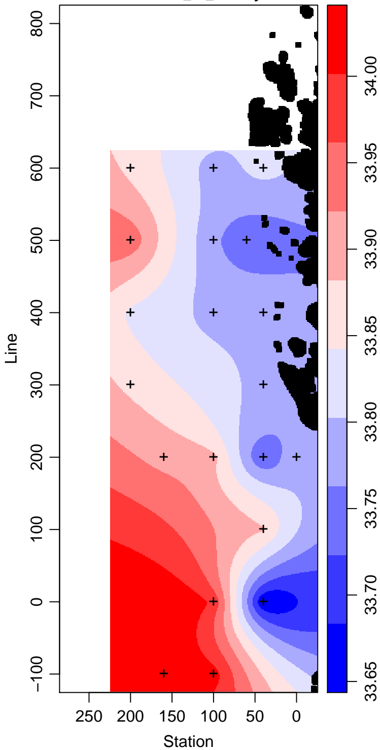
LMG12-01_40_Salinity
