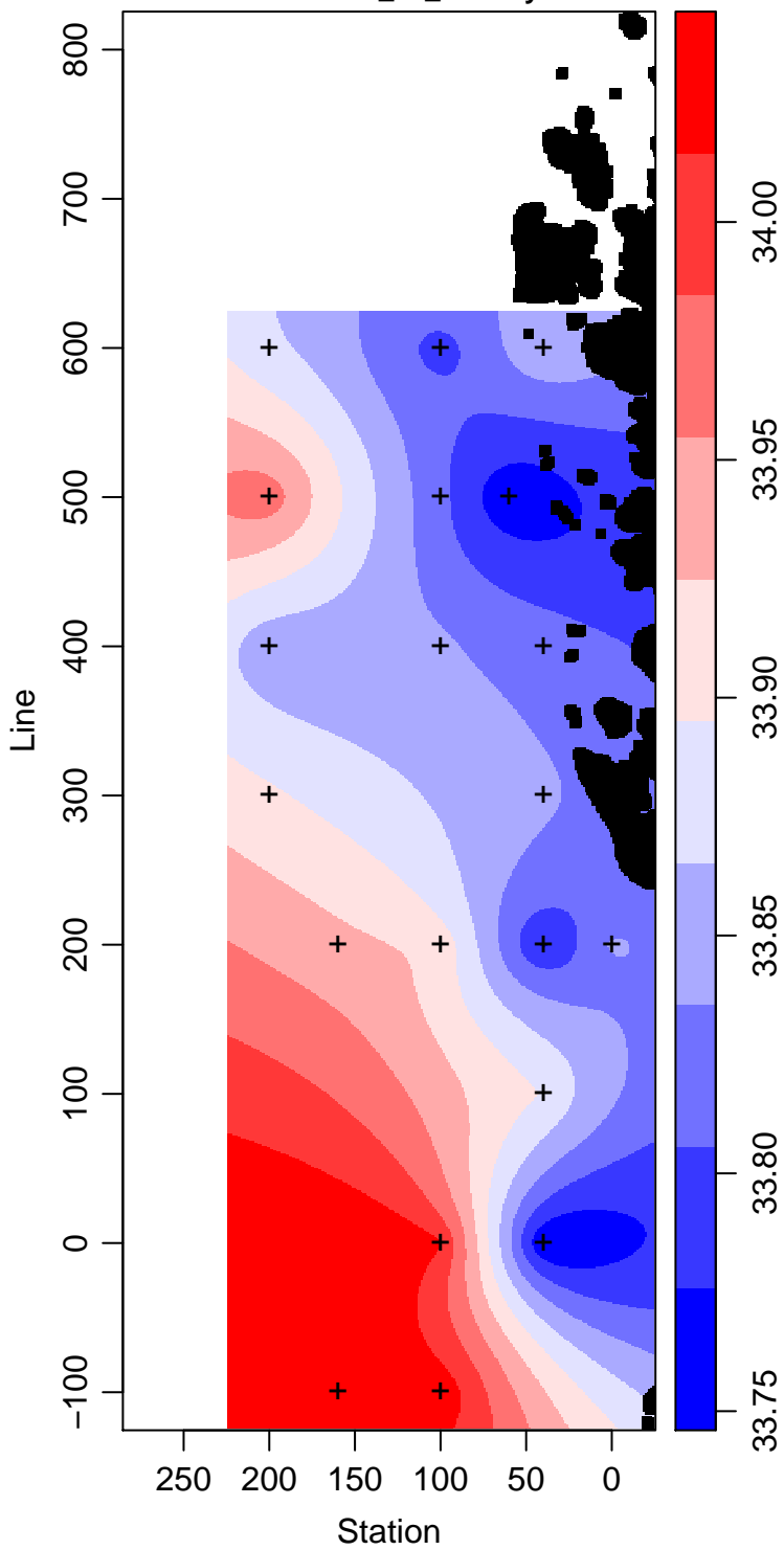
LMG12-01_45_Salinity
