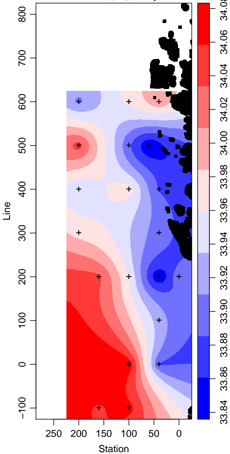
LMG12-01_60_Salinity
