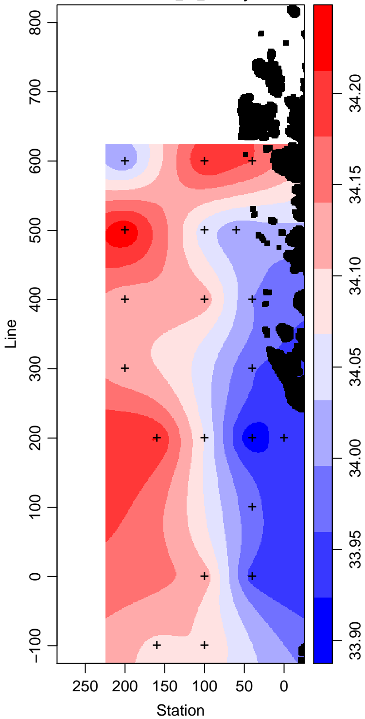
LMG12-01_85_Salinity
