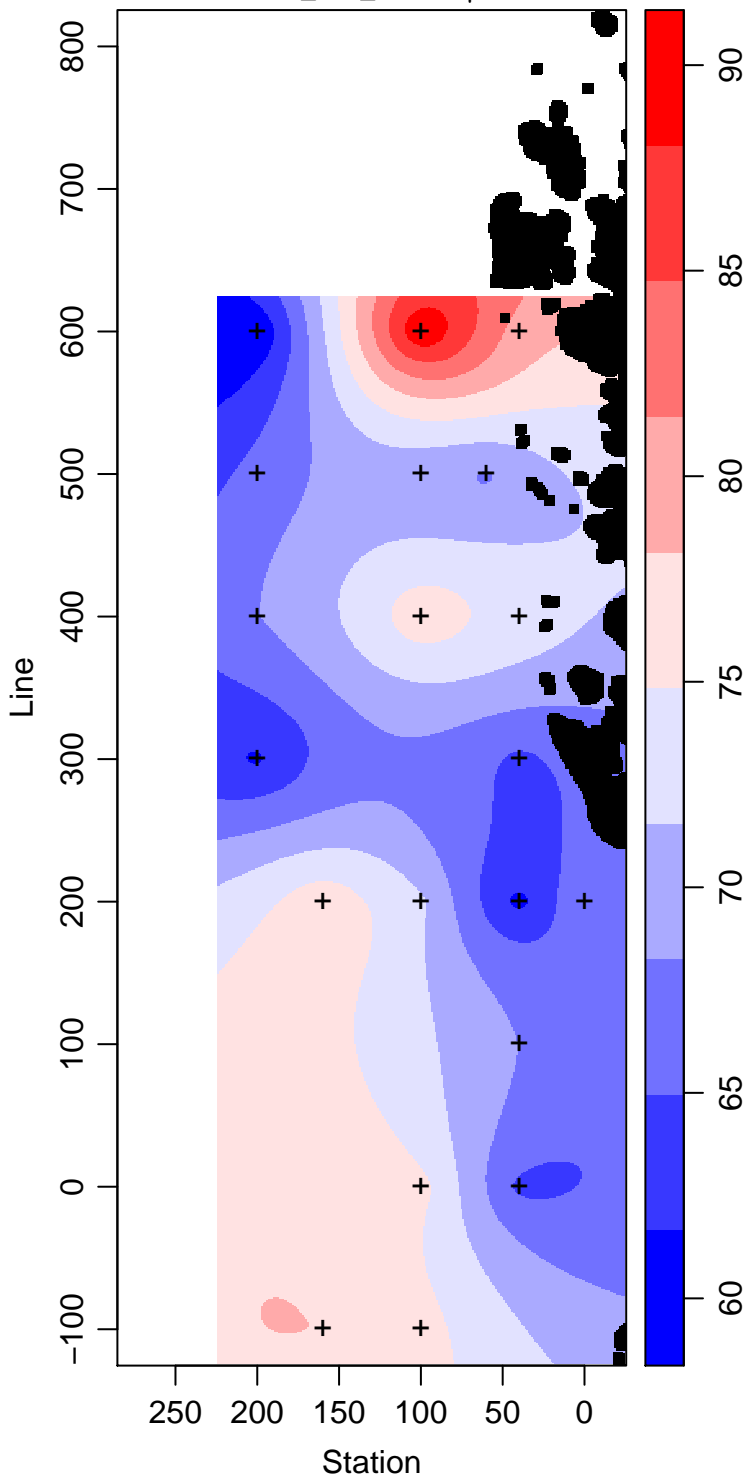
LMG12-01_100_Silicate \mu\text{ mol L}^{-1}
