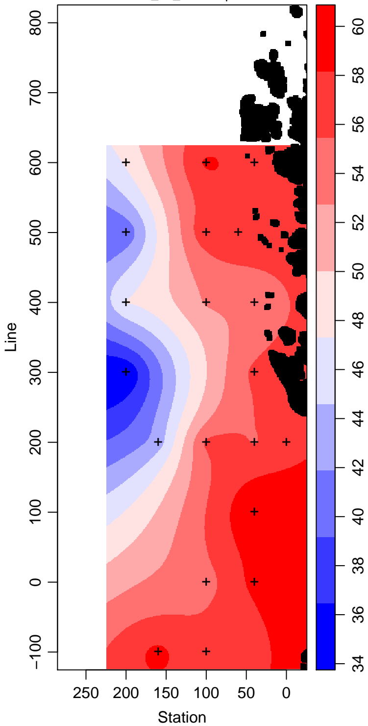
LMG12-01_10_Silicate \mu\text{ mol L}^{-1}
