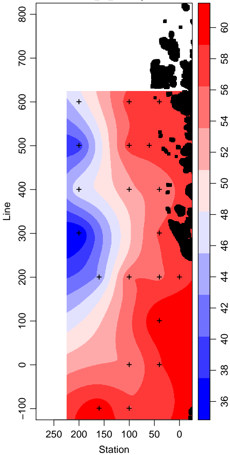
LMG12-01_15_Silicate \mu\text{ mol L}^{-1}
