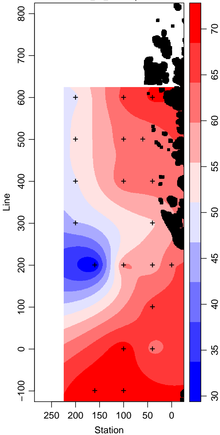
LMG12-01_60_Silicate \mu\text{ mol L}^{-1}
