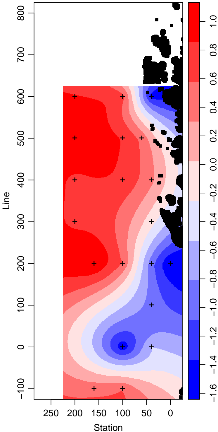
LMG12-01_15_Temperature ° Celsius
