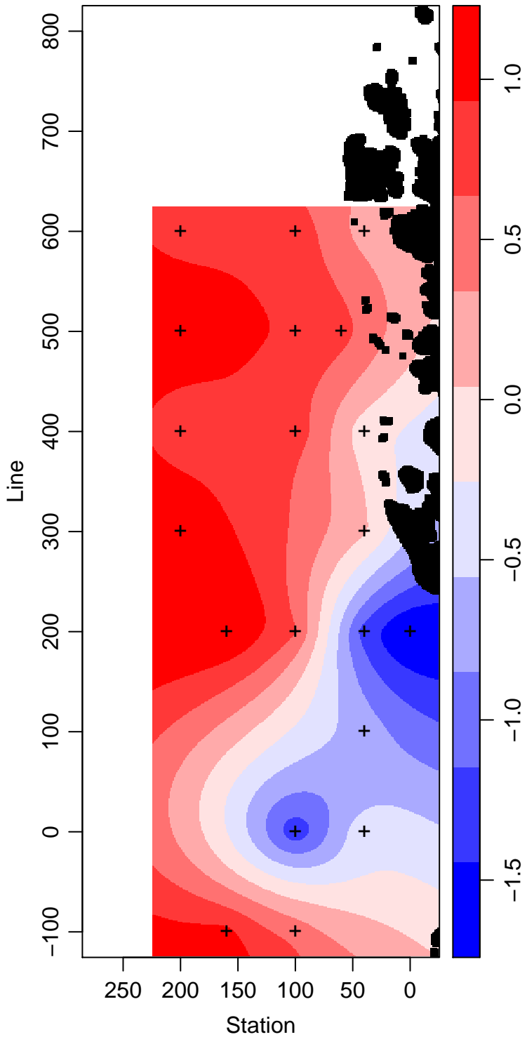
LMG12-01_1_Temperature ° Celsius
