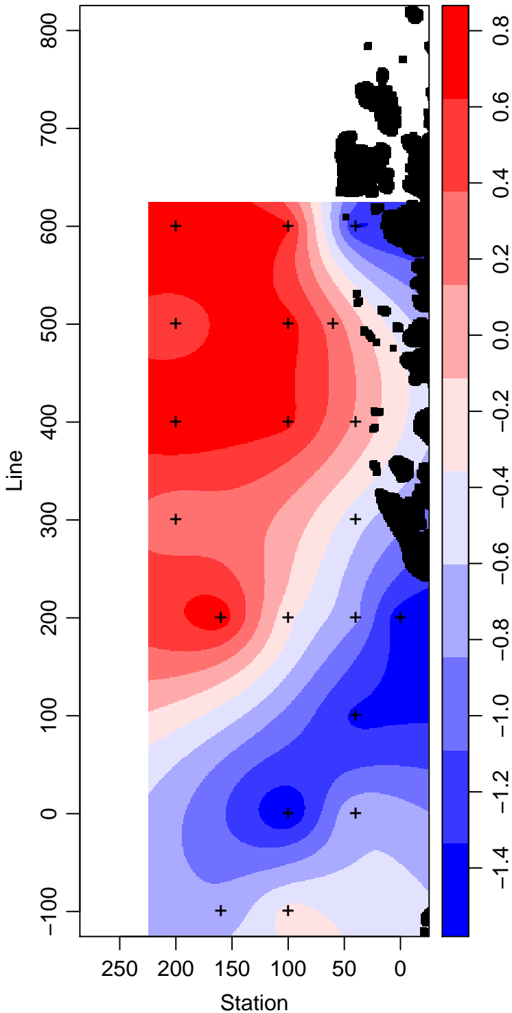
LMG12-01_25_Temperature ° Celsius
