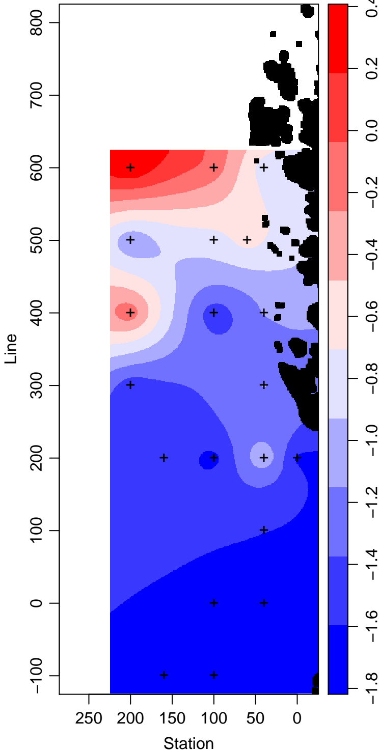
LMG12-01_55_Temperature ° Celsius
