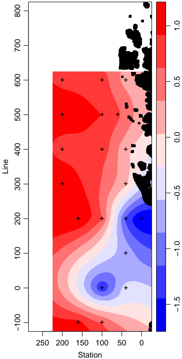
LMG12-01_5_Temperature ° Celsius
