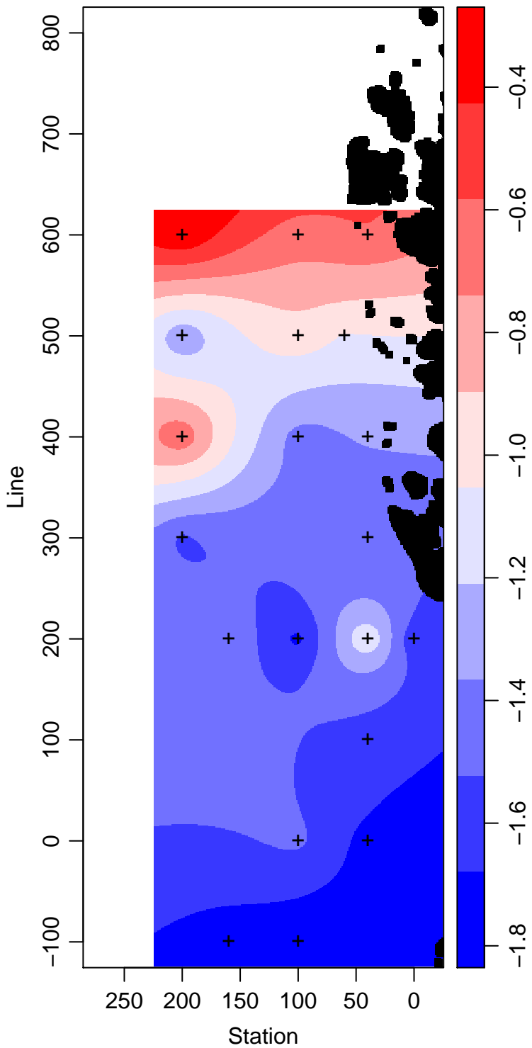
LMG12-01_65_Temperature ° Celsius
