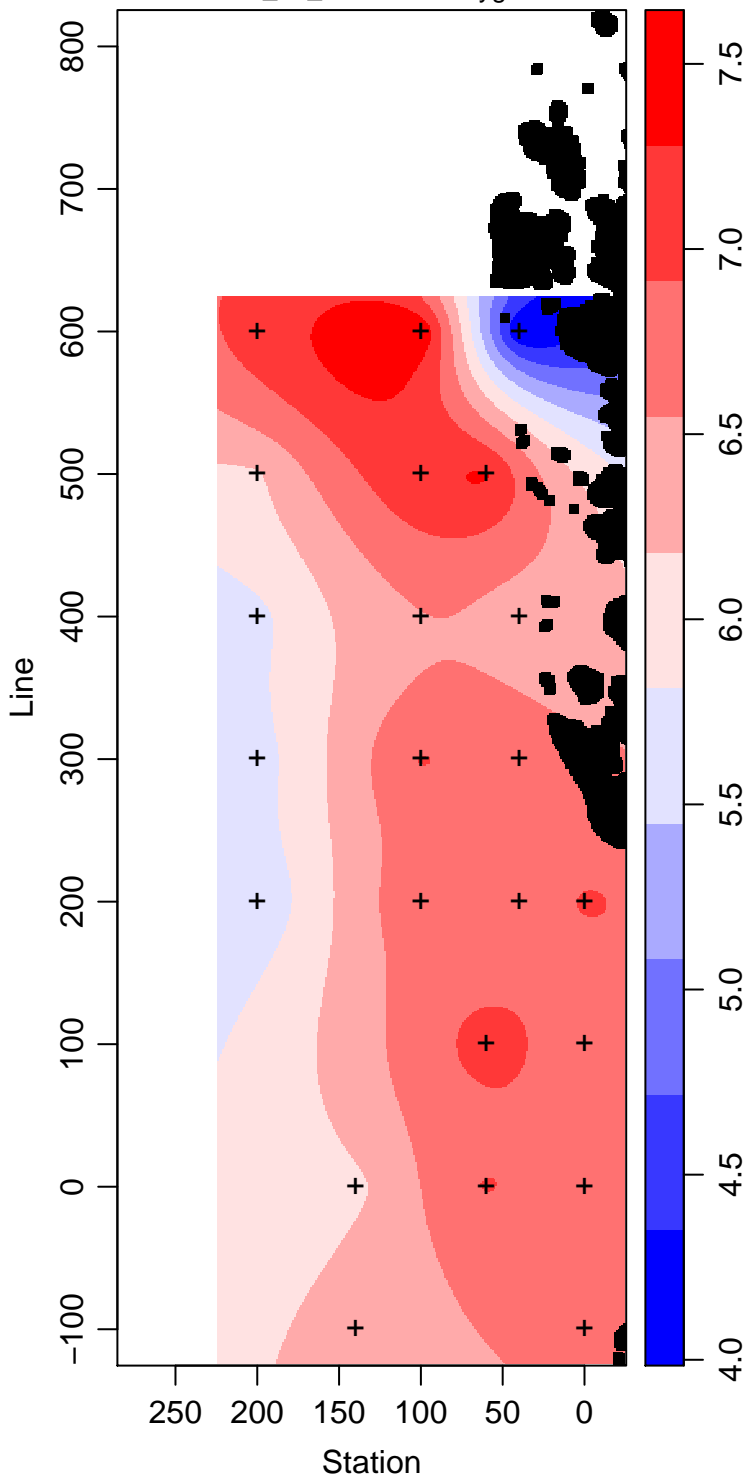
LMG13-01_85_Dissolved.Oxygen ml L -1
