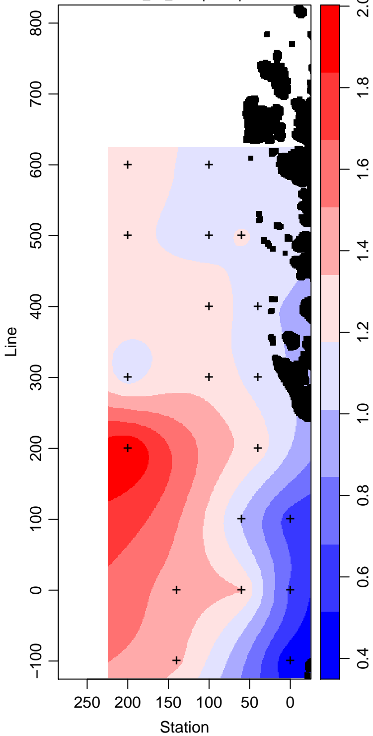
LMG13-01_10_Phosphate \mu\text{ mol L}^{-1}
