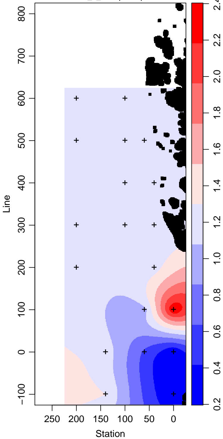
LMG13-01_1_Phosphate \mu\text{ mol L}^{-1}
