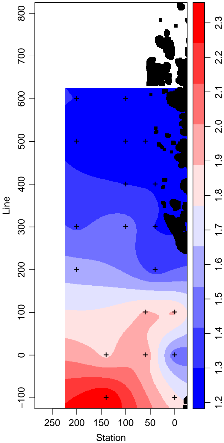
LMG13-01_30_Phosphate \mu\text{ mol L}^{-1}
