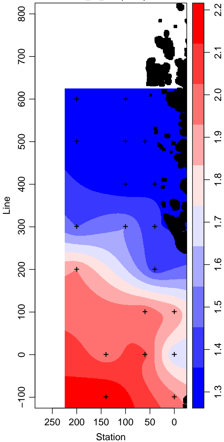
LMG13-01_40_Phosphate \mu\text{ mol L}^{-1}
