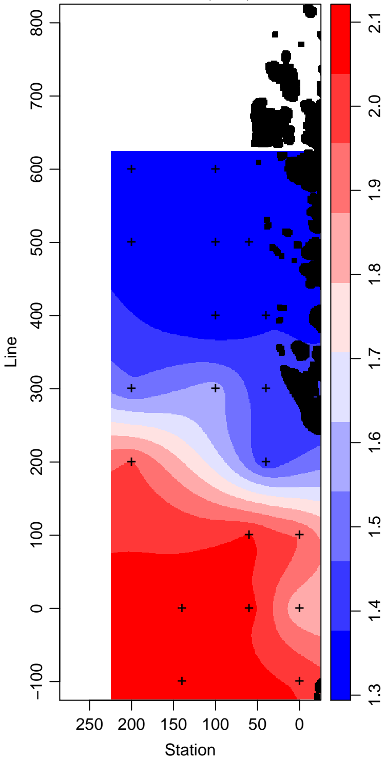
LMG13-01_45_Phosphate \mu\text{ mol L}^{-1}
