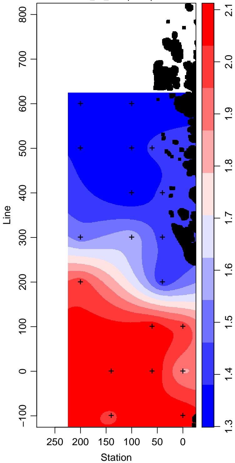
LMG13-01_50_Phosphate \mu\text{ mol L}^{-1}
