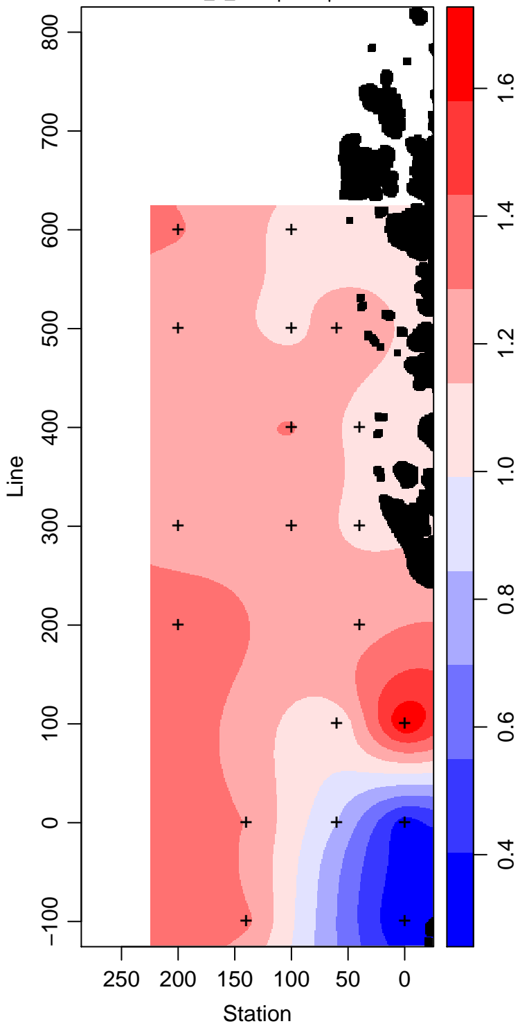
LMG13-01_5_Phosphate \mu\text{ mol L}^{-1}
