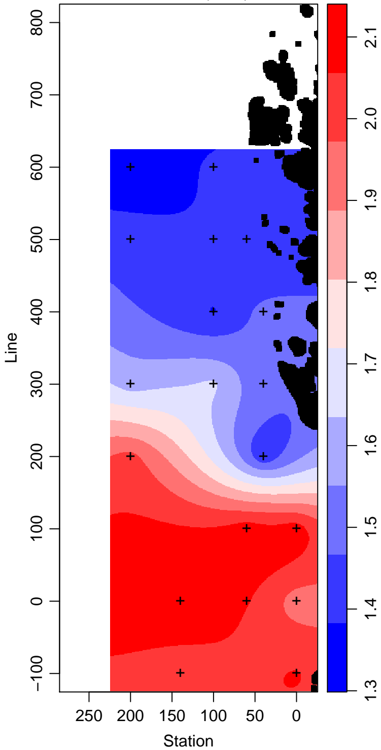
LMG13-01_60_Phosphate \mu\text{ mol L}^{-1}
