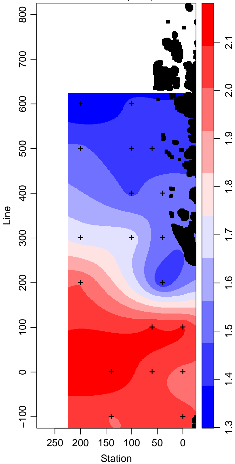
LMG13-01_70_Phosphate \mu\text{ mol L}^{-1}
