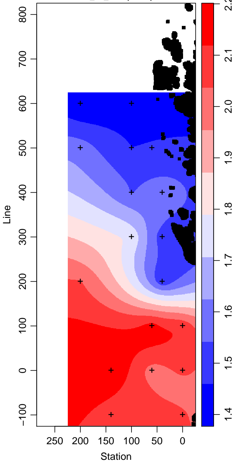
LMG13-01_85_Phosphate \mu\text{ mol L}^{-1}
