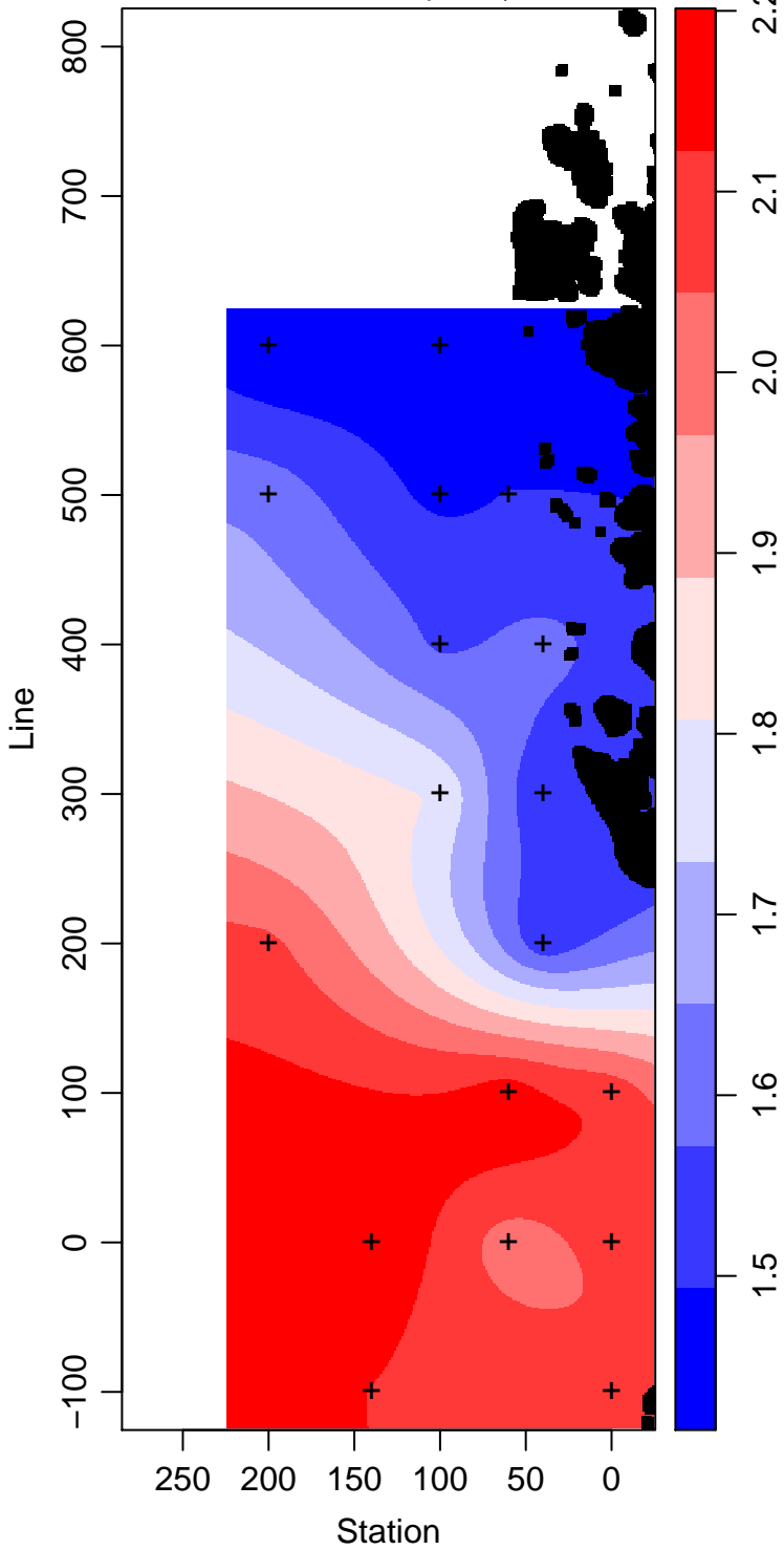
LMG13-01_90_Phosphate \mu\text{ mol L}^{-1}
