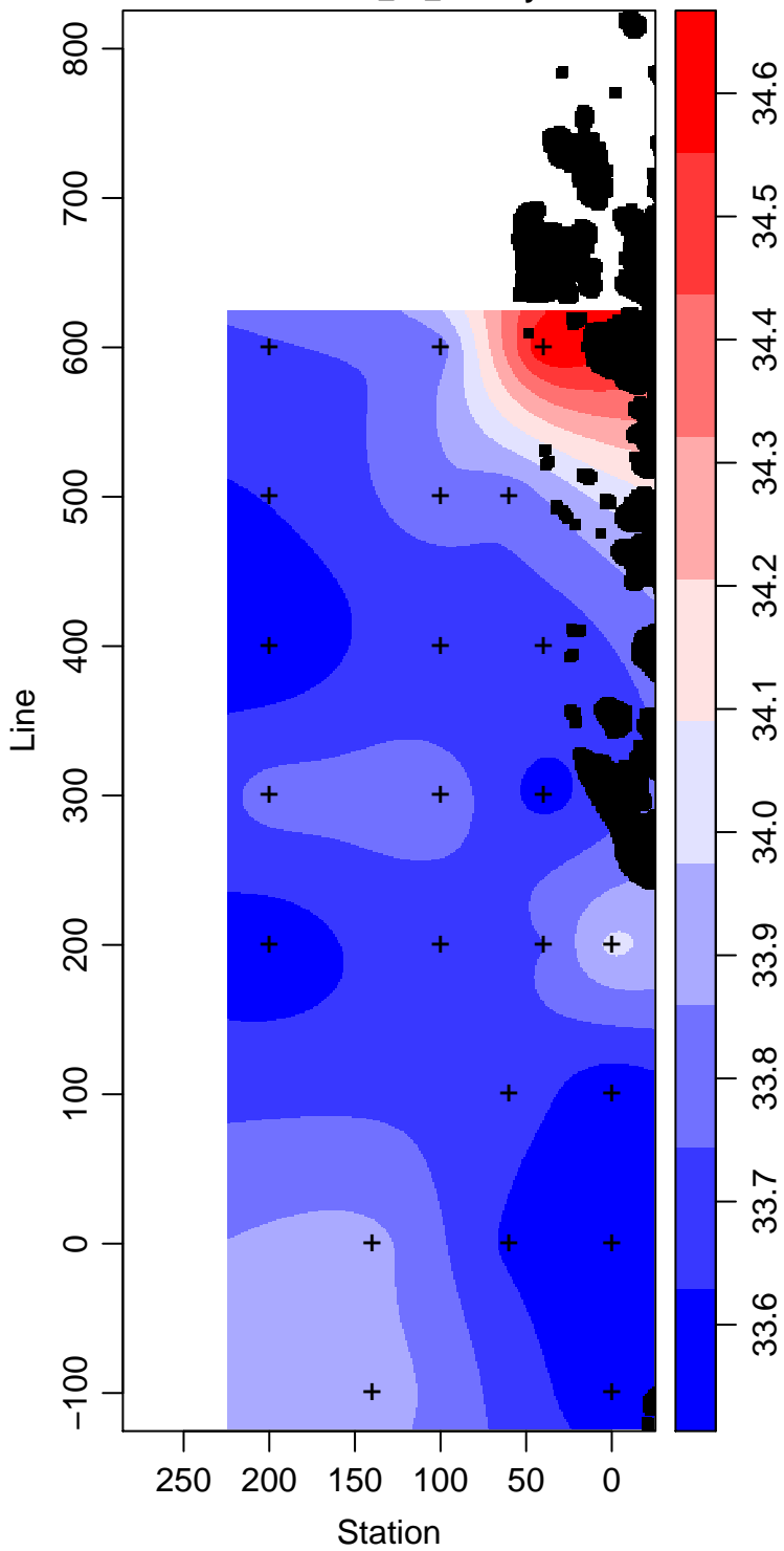
LMG13-01_25_Salinity
