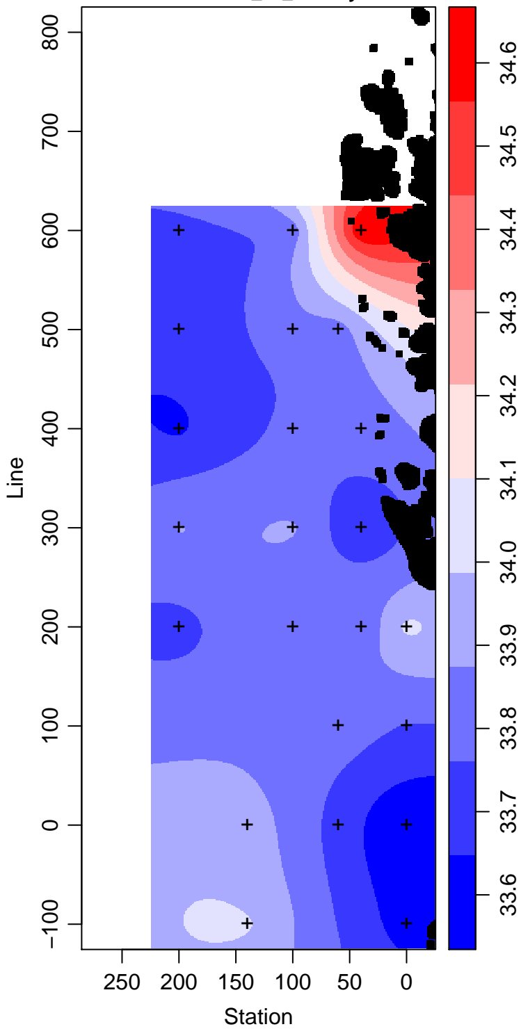
LMG13-01_30_Salinity
