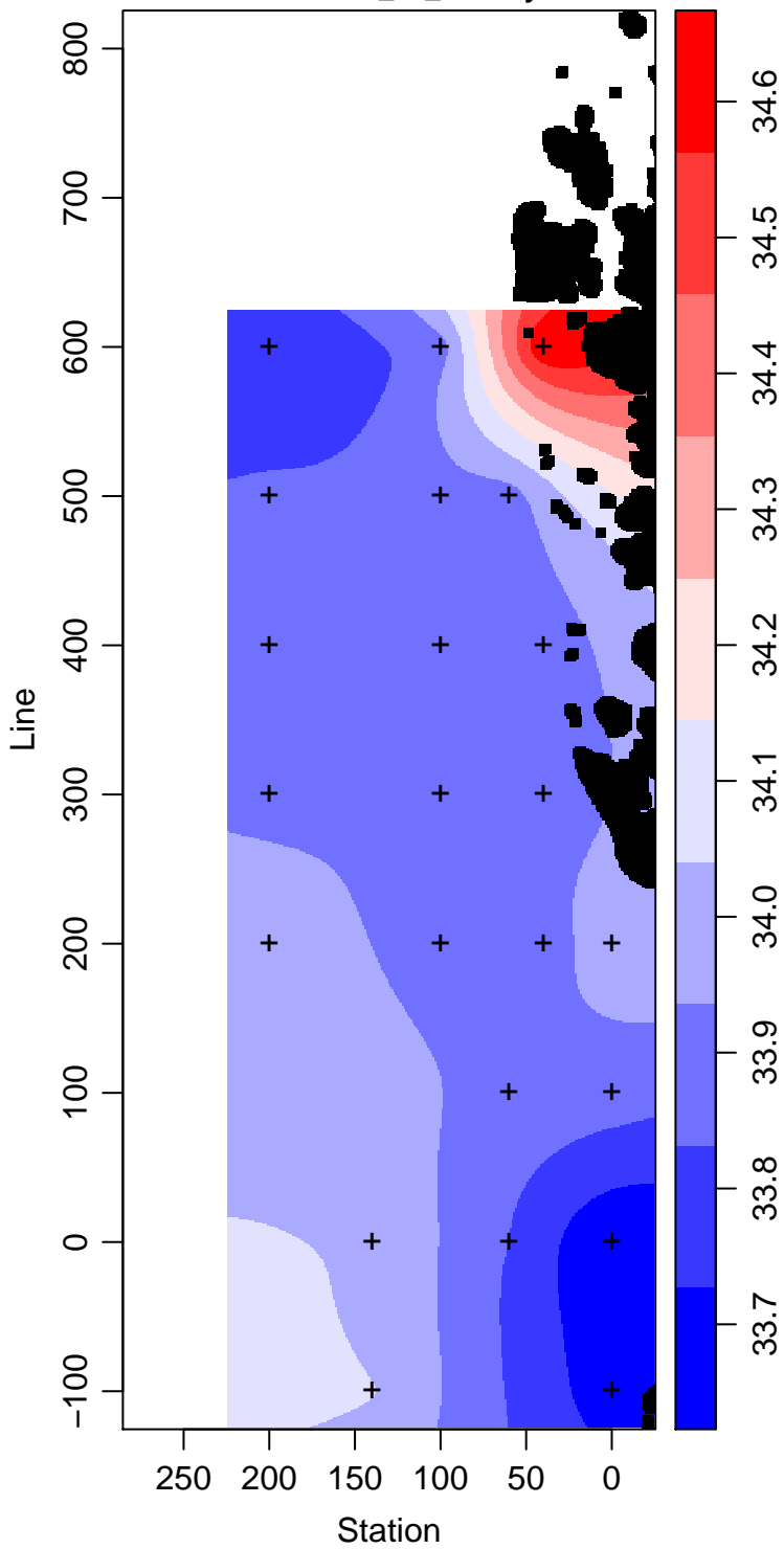
LMG13-01_45_Salinity
